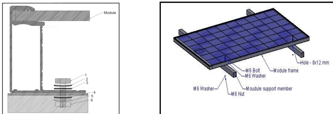
Fig: Mounting Details-1
