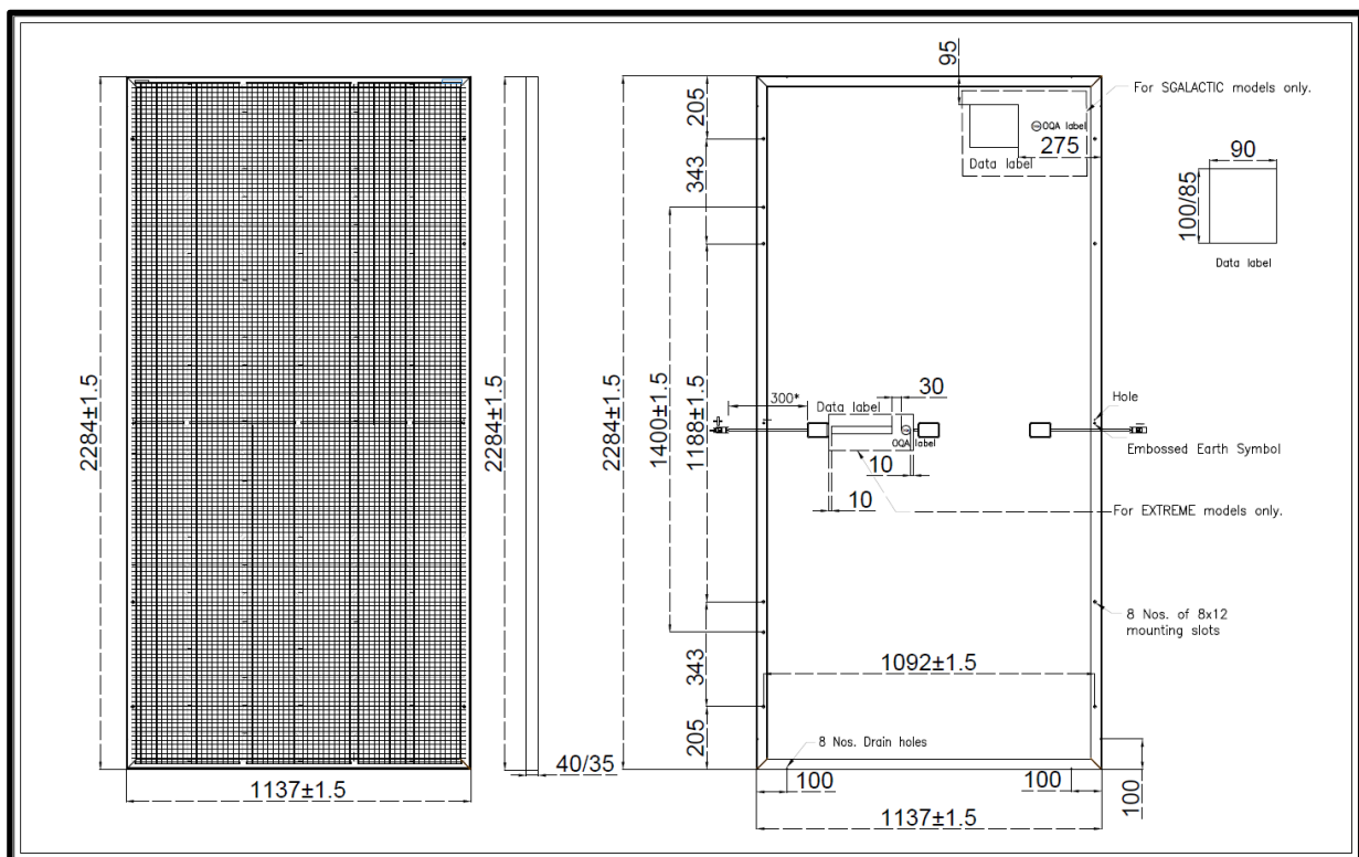
Fig: Finished Module Details (For Reference only)
