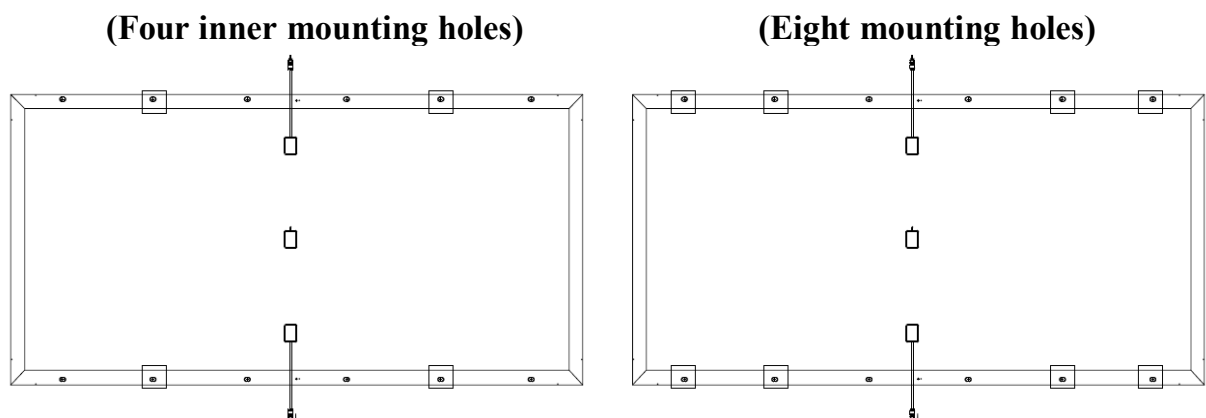
Fig: Mounting Details-1
