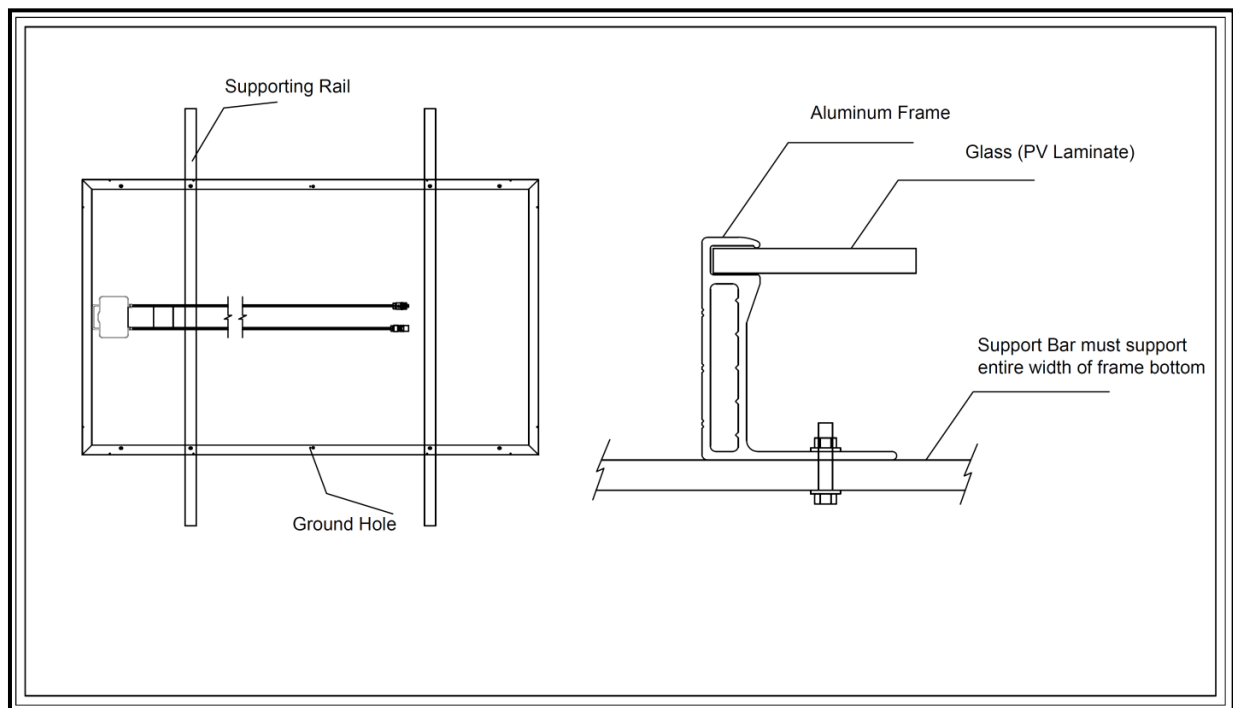
Fig: Mounting Details-3
